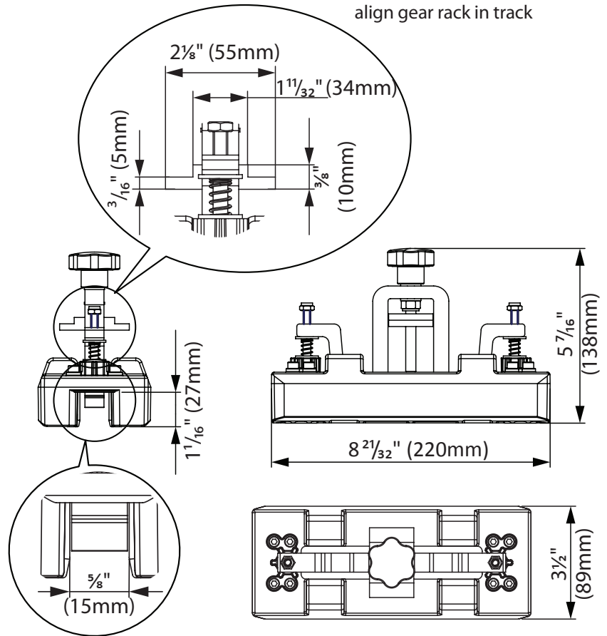
The Integrator Gear Rack Installation Tool
